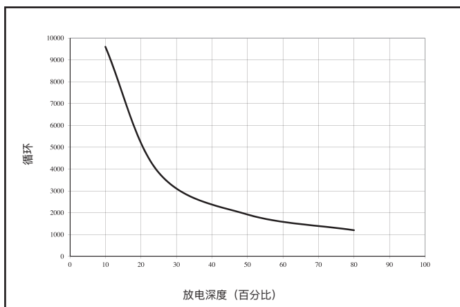
循环寿命与放电深度@ +25°C (77°F)*
